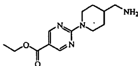
intermediate 4
